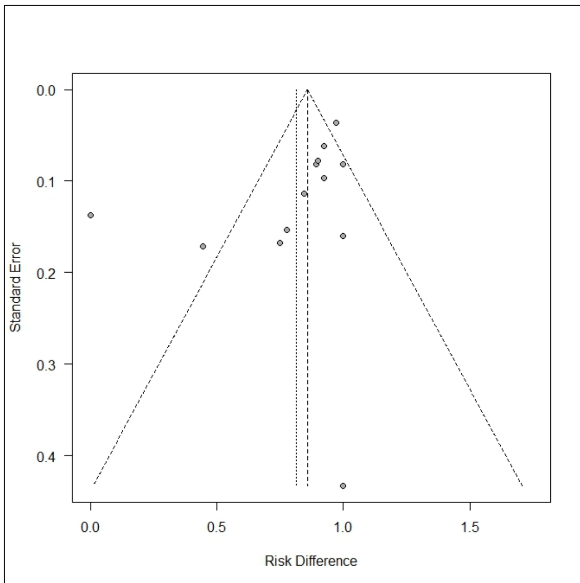
Supplementary Figure 3. Funnel plot of probability of BRAF^{V600E} (-) in metastatic lesion of melanoma against BRAF^{V600E} (-) in primary lesion.
